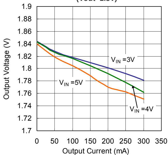
Output Voltage vs. Output Current (Vout=1.8V)
