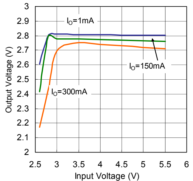
Output Voltage vs. Input Voltage (Vout=2.8V)
