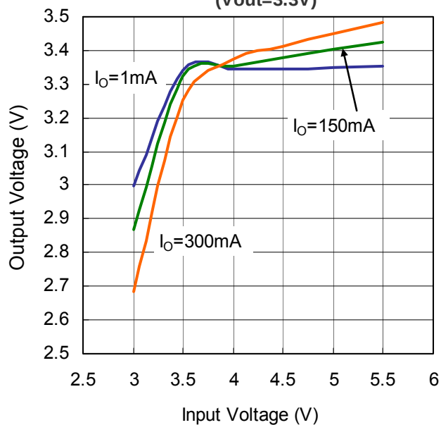
Output Voltage vs. Input Voltage (Vout=3.3V)
