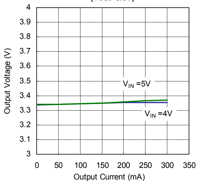
Output Voltage vs. Output Current (Vout=3.3V)
