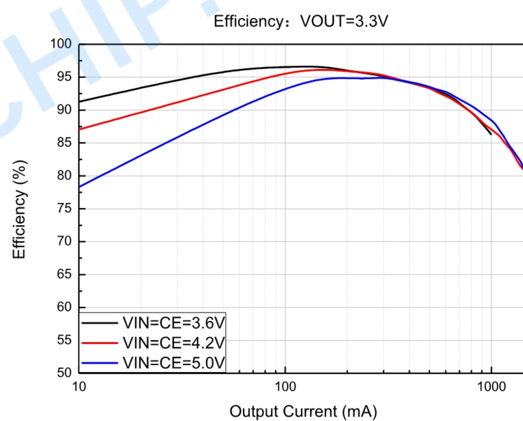
效率 @ VOUT=3.3V
