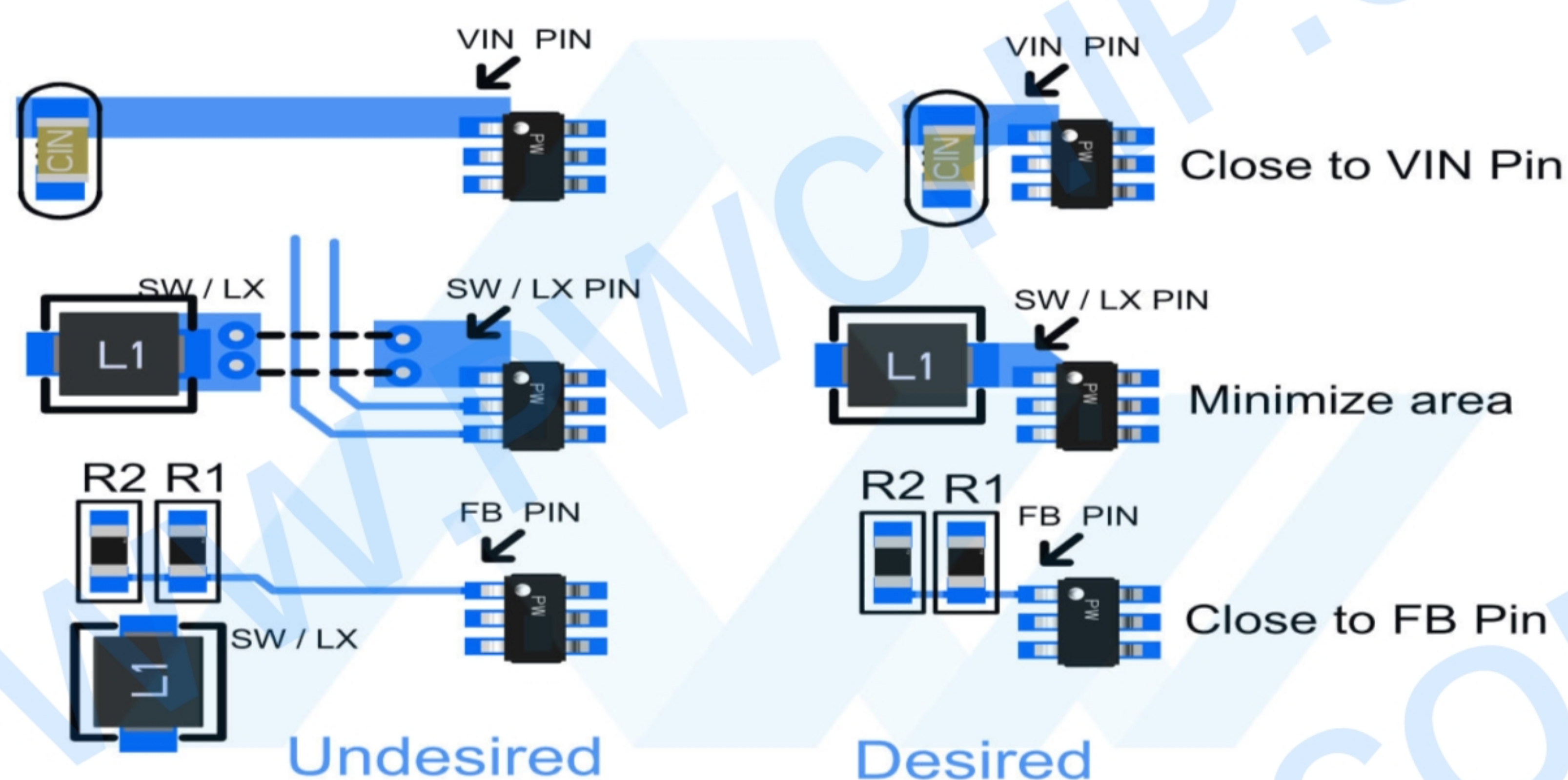
PCB layout
