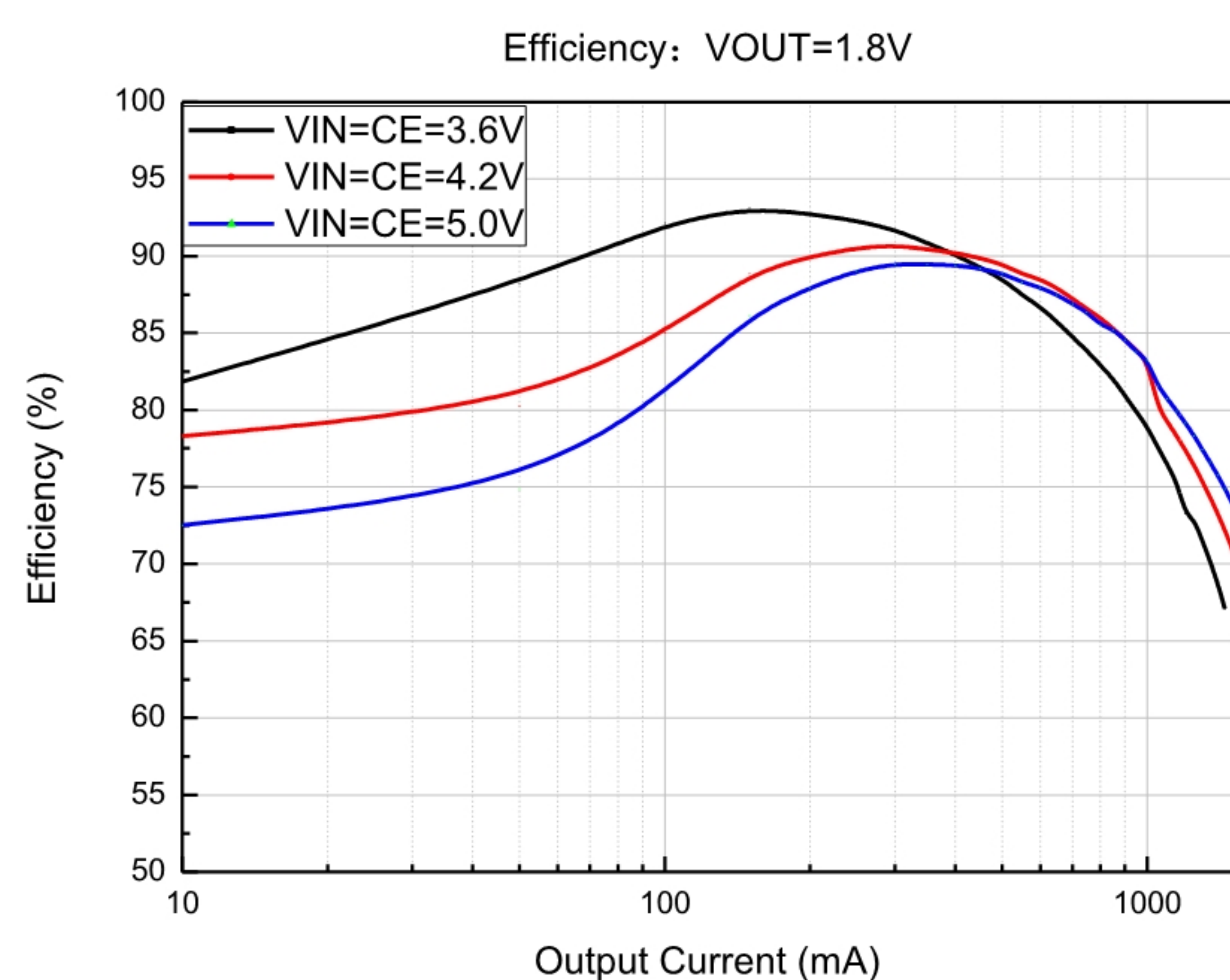
效率 @ VOUT=1.8V
