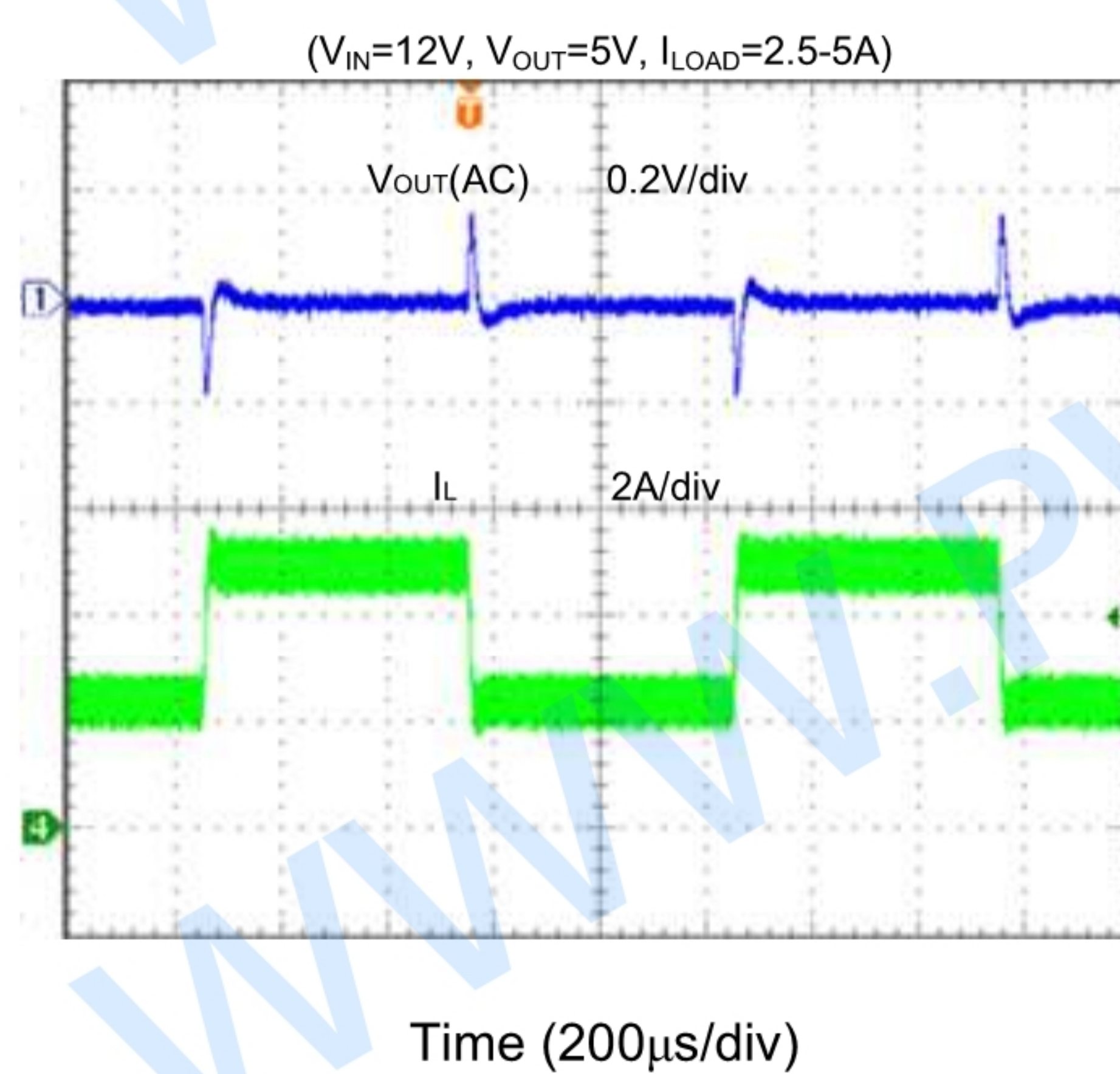
Load Transient
