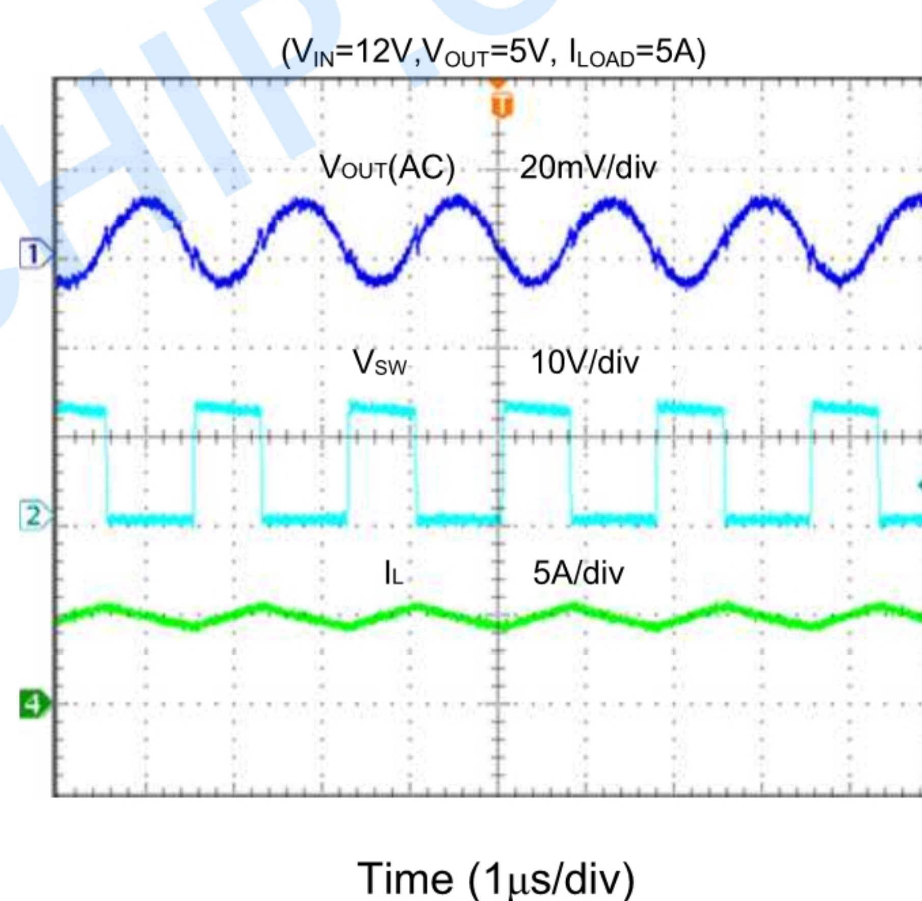
Output Ripple
