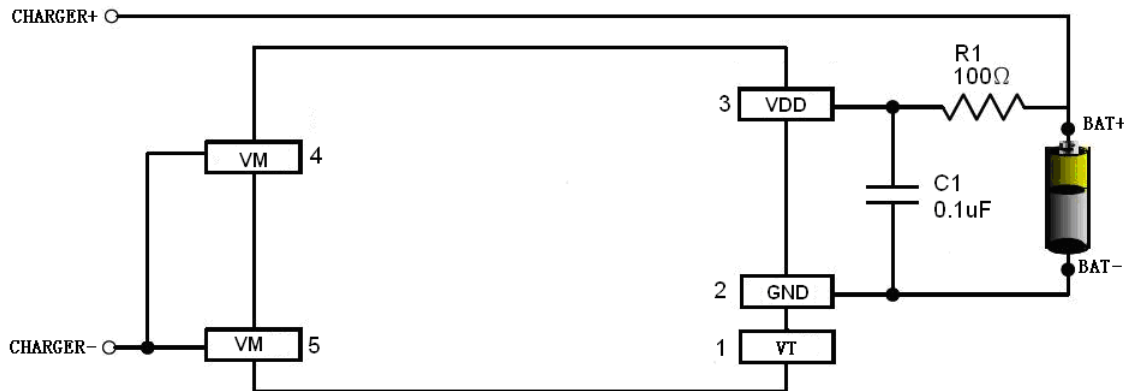
Fig 6 SD5358A in a Typical Battery Protection Circuit
