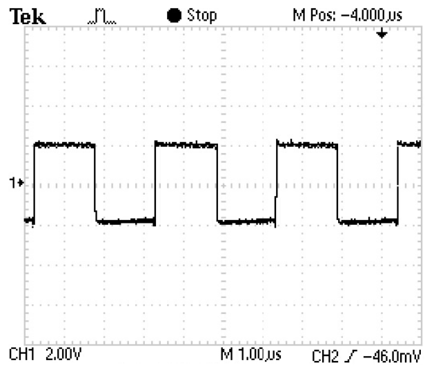
SW Noise (V IN =4.2V, I LOAD =100mA)
