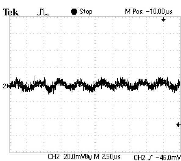
Output Noise (V IN =4.2V, I LOAD =100mA)
