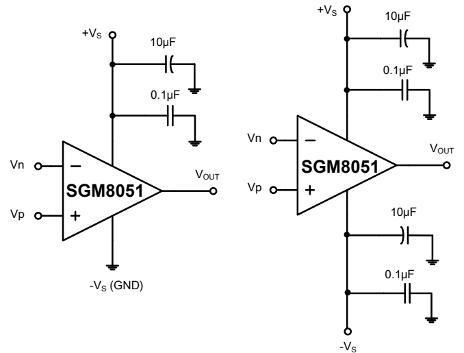
Figure 2. Amplifier with Bypass Capacitors
