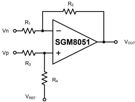
Figure 3. Differential Amplifier
