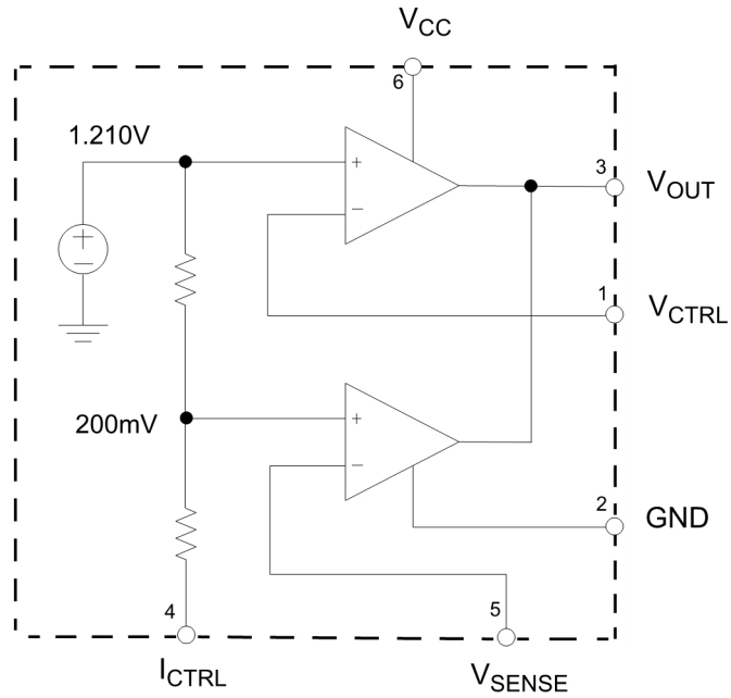
Figure 3. Functional Block Diagram of PL4313
