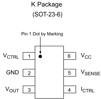
Figure 2. Pin Configuration of PL4313 (Top View)
