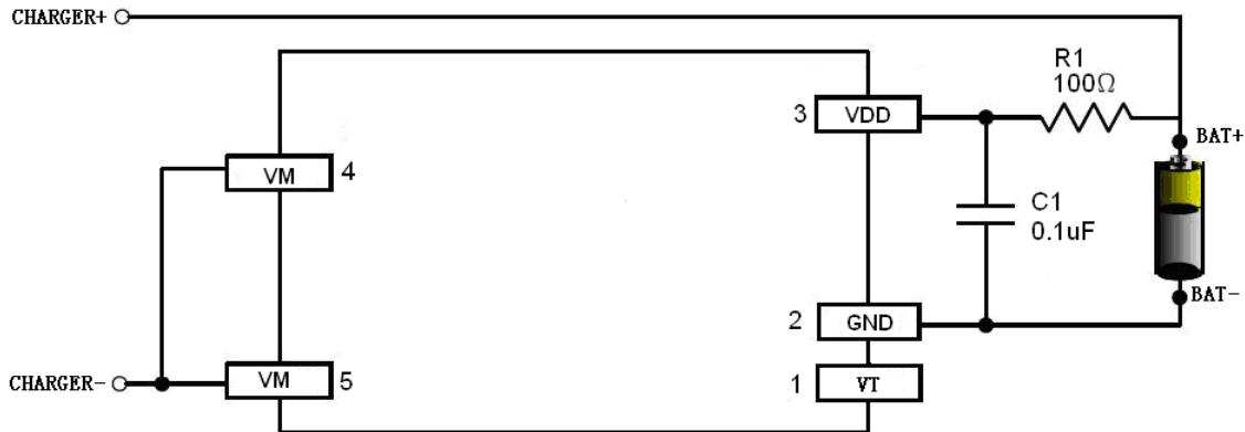
Fig 6 PL5358 in a Typical Battery Protection Circuit
