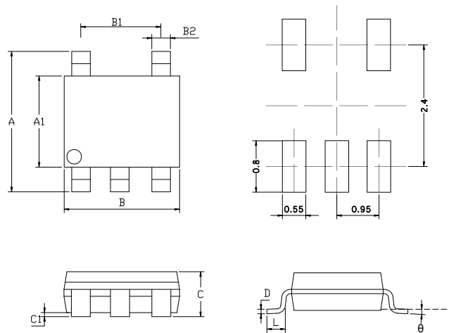
SOT23-5 package mechanical drawing
