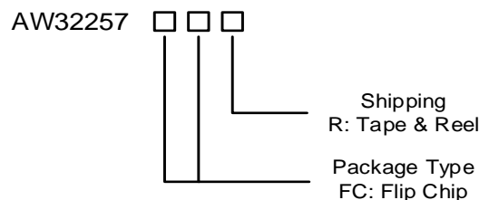
Figure 3 Package Information
