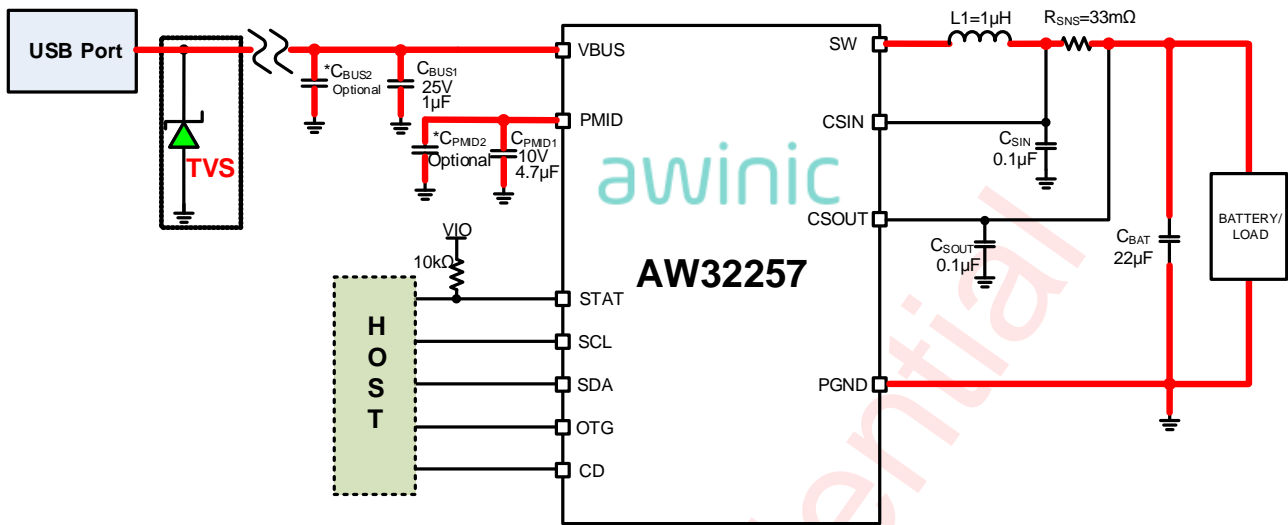
Figure 4 AW32257 Application Circuit
