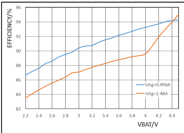
V_{BUS}=5V , DCR of Inductor is 23m\Omega Figure 13 Charge efficiency vs. VBAT
