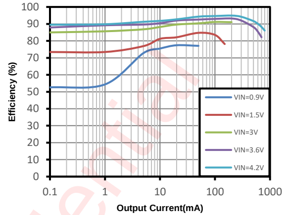
AW360997 Load Efficiency with Different Inputs
