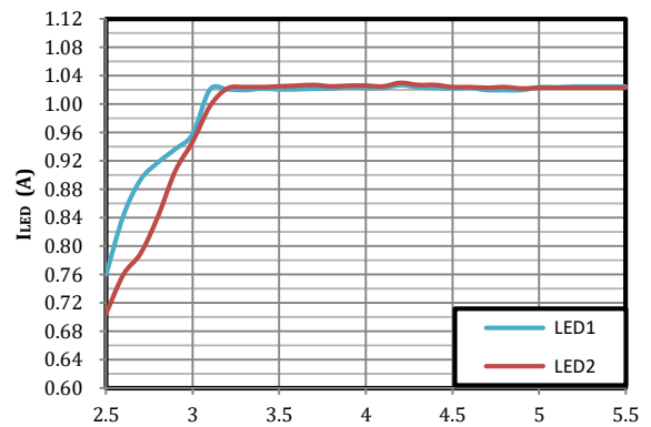
LED1 & LED2 Current vs Input Voltage
