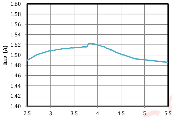
LED1/2 Flash Current vs Input Voltage
