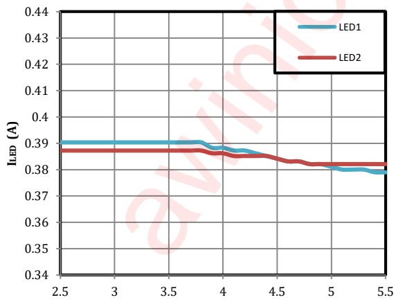
I LED =0.386A fsw=2MHz Torch LED1&2 Torch Current vs Input Voltage
