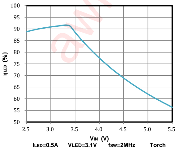
I_{LED}=0.5A V_{LED}=3.1V f_{sw}=2MHz Torch LED Efficiency vs Input Voltage
