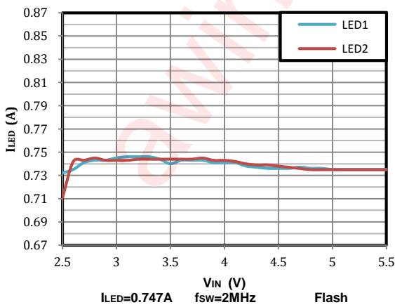
LED1 & LED2 Current vs Input Voltage
