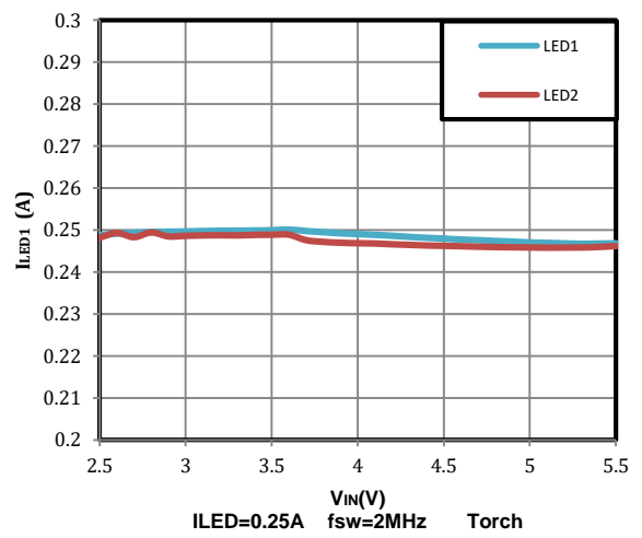
LED1&2 Torch Current vs Input Voltage
