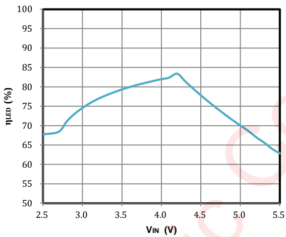
I_{LED}=1.5A V_{LED}=3.5V f_{sw}=2MHz Flash LED Efficiency vs Input Voltage
