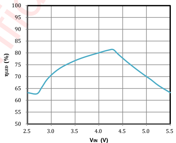
I_{LED}=1.5A V_{LED}=3.5V f_{sw}=4MHz Flash LED Efficiency vs Input Voltage
