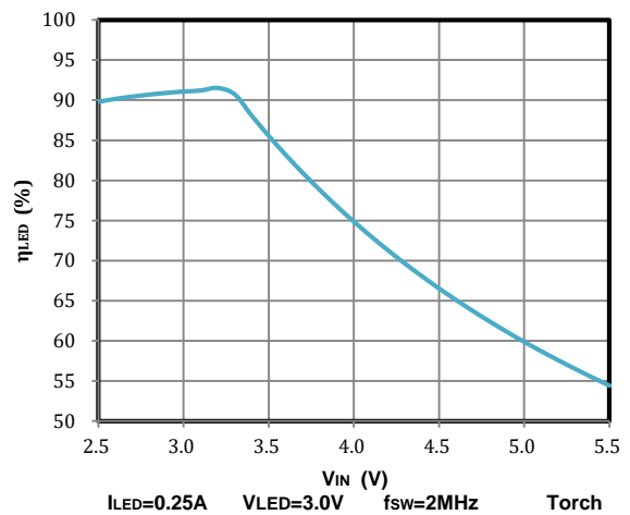
I_{LED}=0.25A V_{LED}=3.0V f_{sw}=2MHz Torch LED Efficiency vs Input Voltage
