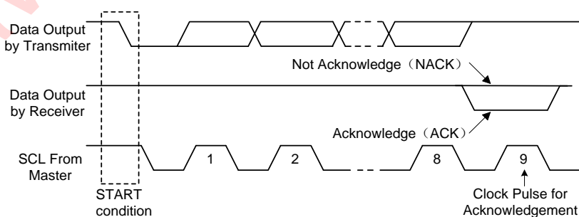
Fig 34 Acknowledgement Diagram
