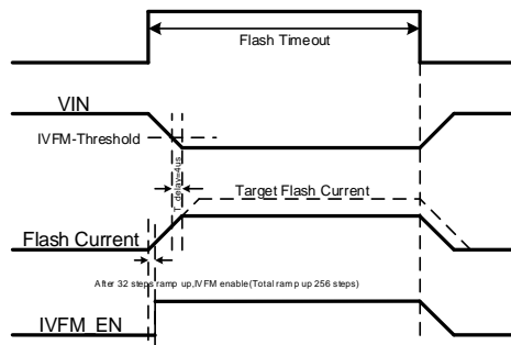
Fig 31 IVFM Timing
