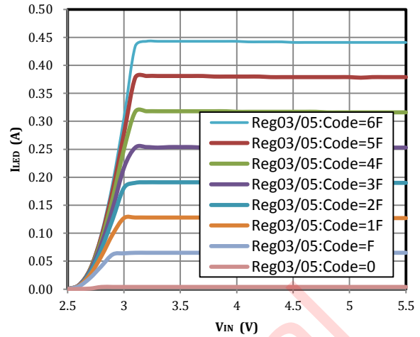
Fig 12. LED1/2 Flash Current vs Input Voltage
