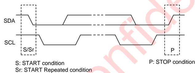
Fig 33 Start and Stop Conditions
