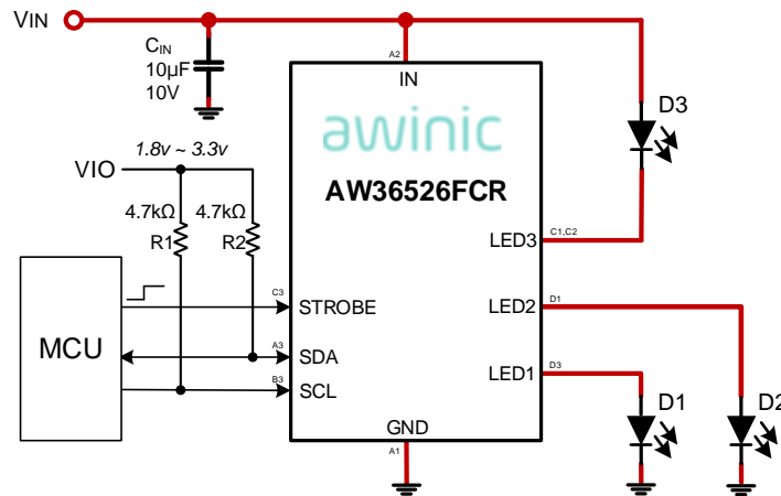
Fig 3 AW36526 Application Circuit
