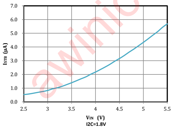
Fig 21. Standby Current vs Input Voltage
