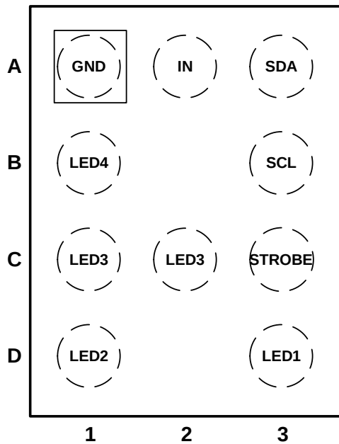
AW36529FCR Pin Configuration (Top View)
