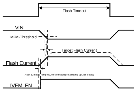
Fig 33 IVFM Timing
