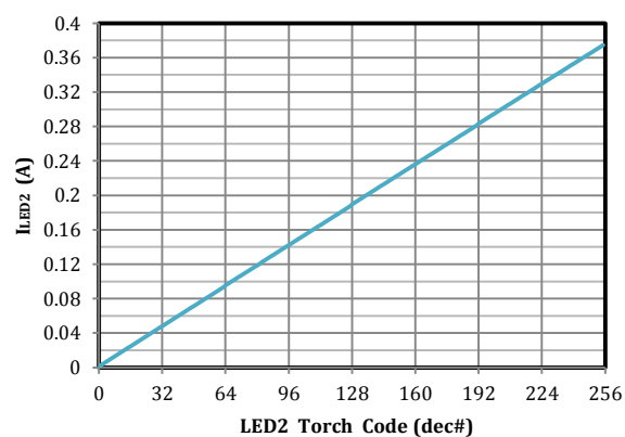
Fig10. LED2 Torch Current vs Brightness Code
