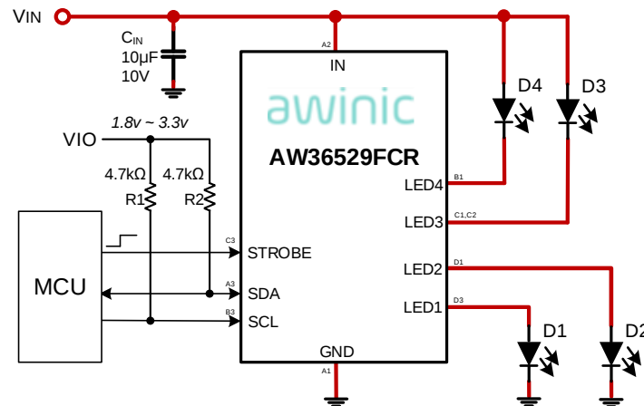
Fig 3 AW36529 Application Circuit
