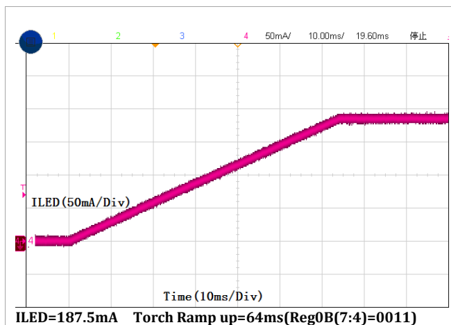
Fig 29. Torch Ramp up time
