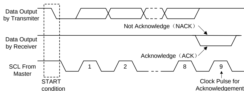
Fig 36 Acknowledgement Diagram
