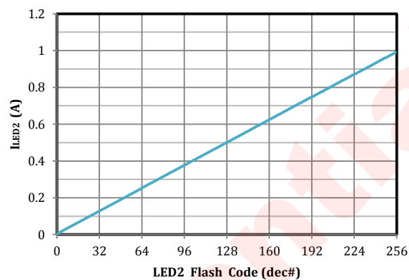
Fig6. LED2 Flash Current vs Brightness Code
