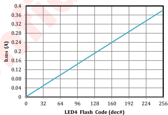
Fig8. LED4 Flash Current vs Brightness Code
