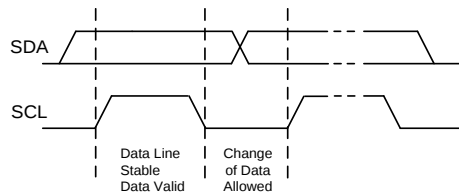
Fig 34 Data Validation Diagram
