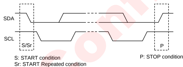
Fig 35 Start and Stop Conditions
