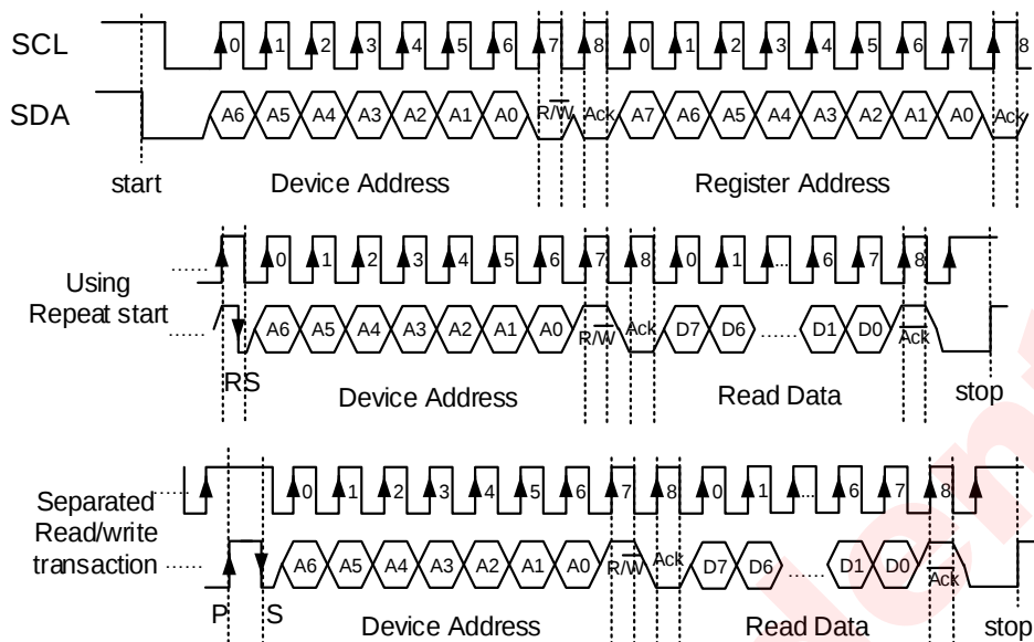
Fig 38 I 2 C Read Timing
