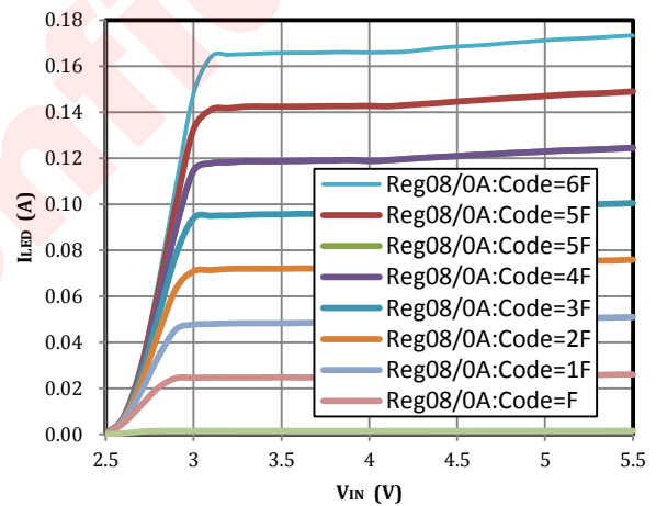
Fig20. LED3/4 Torch Current vs Input Voltage
