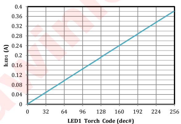
Fig9. LED1 Torch Current vs Brightness Code
