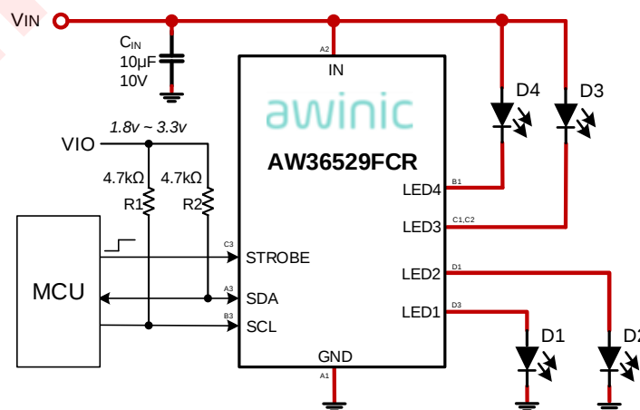
Fig 1 Typical Application Circuit of AW36529
