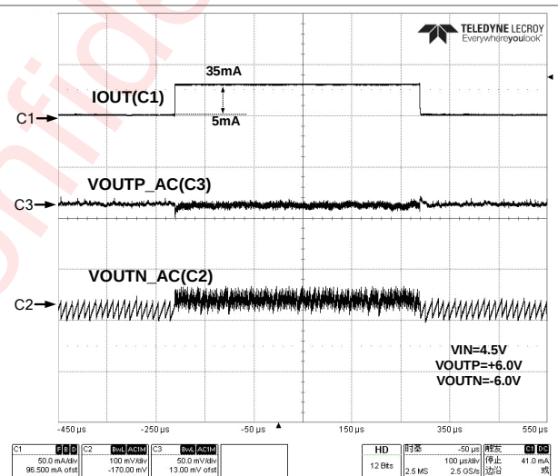
Figure 50 Load Transient (40mA Mode)
