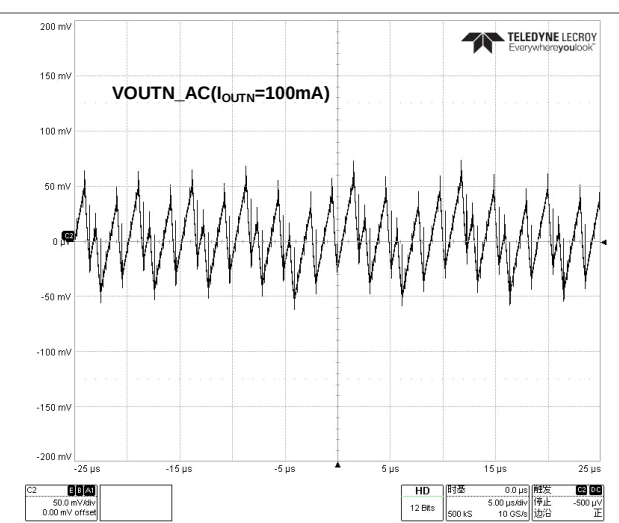
Figure 46 V OUTN Output Voltage Ripple(100mA Mode)
