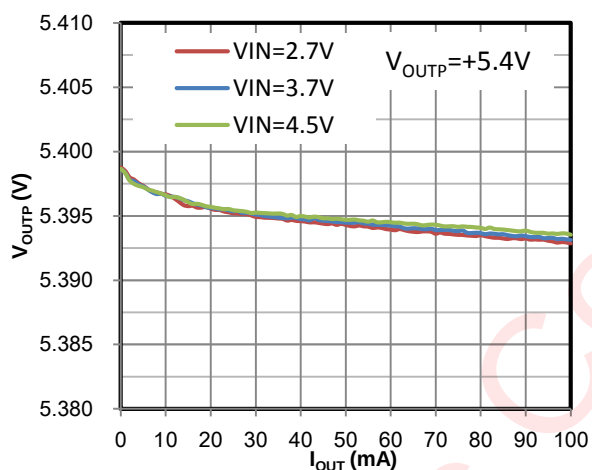
Figure 37 Load Regulation (100mA Mode)
