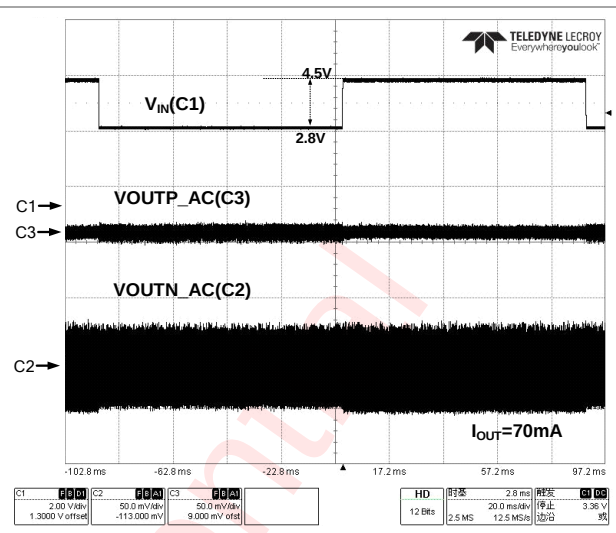
Figure 60 Line Transient (80mA Mode)
