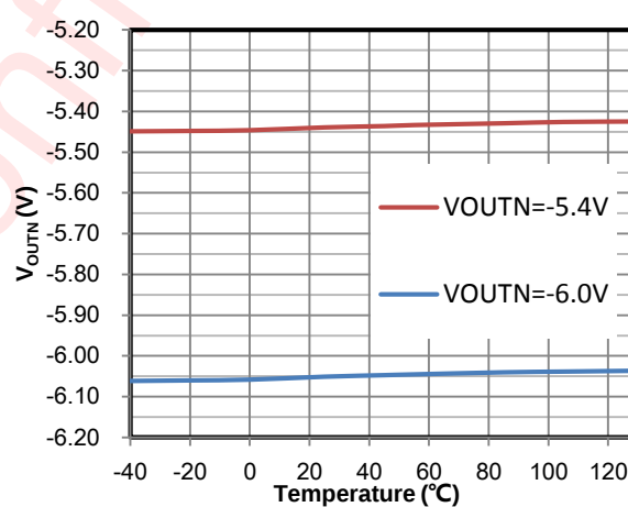
Figure 9 V_{OUTN} vs. Temperature
