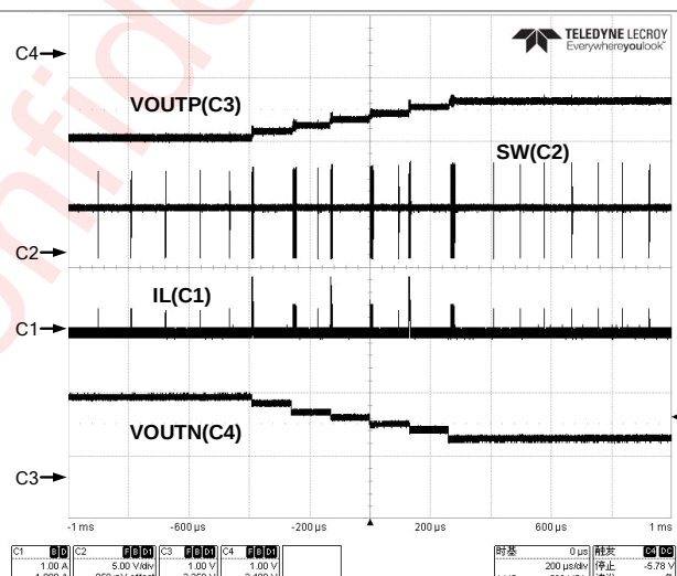
Figure 74 Ramp Up ( V_{OUTP} And V_{OUTN} )
