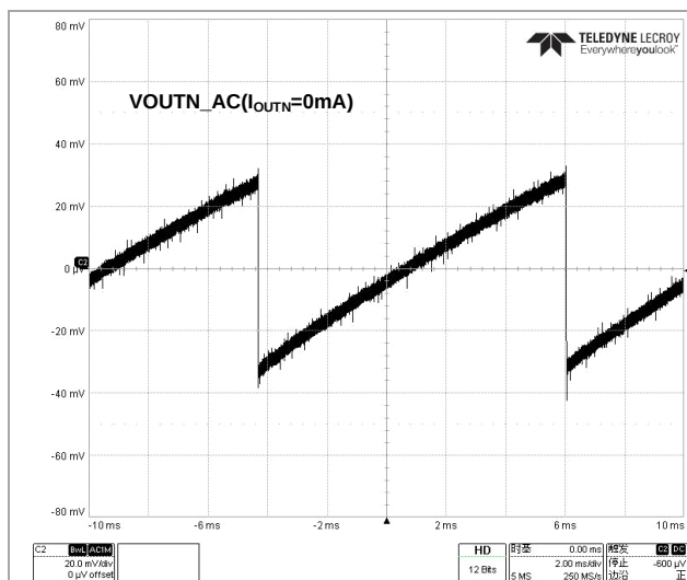
Figure 41 V OUTN Output Voltage Ripple (80mA Mode)
