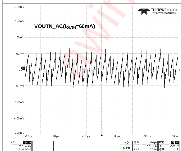
Figure 45 V OUTN Output Voltage Ripple(100mA Mode)
