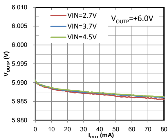
Figure 35 Load Regulation (80mA Mode)
