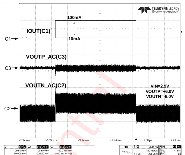
Figure 54 Load Transient (100mA Mode)
