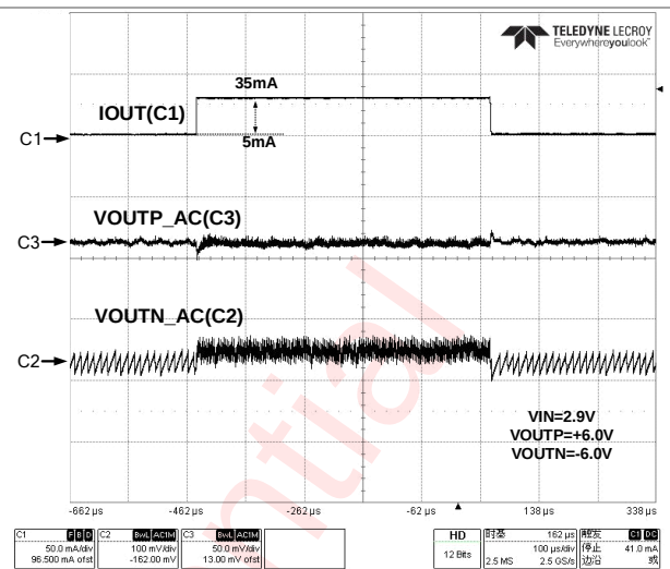
Figure 48 Load Transient (40mA Mode)
