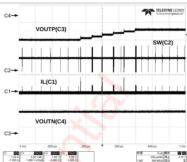
Figure 72 Ramp Up ( V_{OUTP} )
