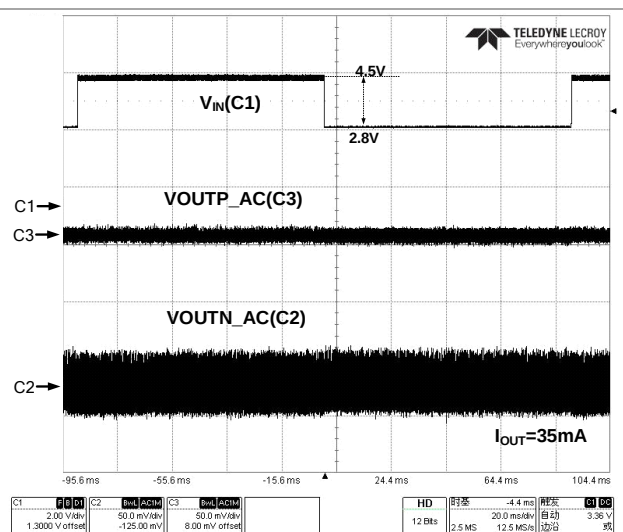
Figure 58 Line Transient (40mA Mode)
