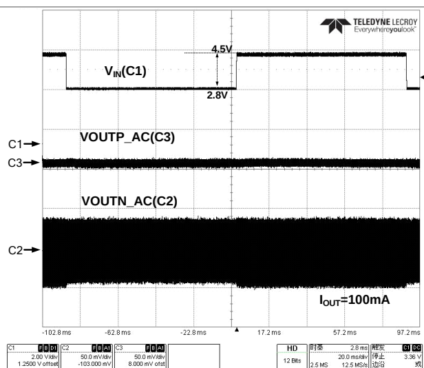
Figure 64 Line Transient (100mA Mode)
