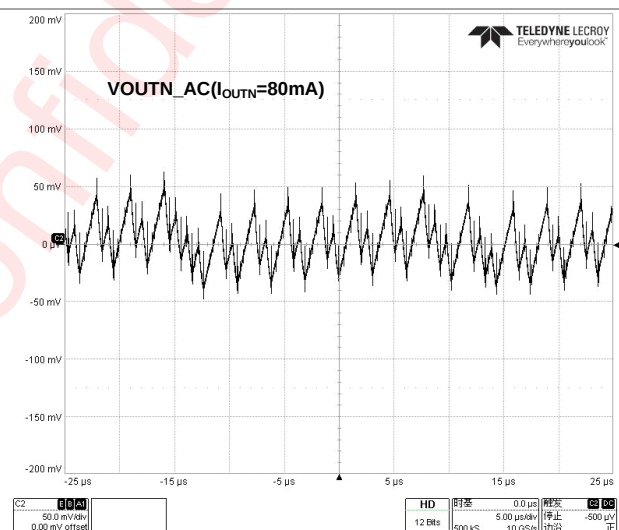
Figure 44 V OUTN Output Voltage Ripple(80mA Mode)
