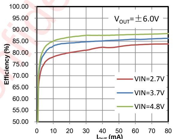
Figure 14 Efficiency (80mA Mode)
