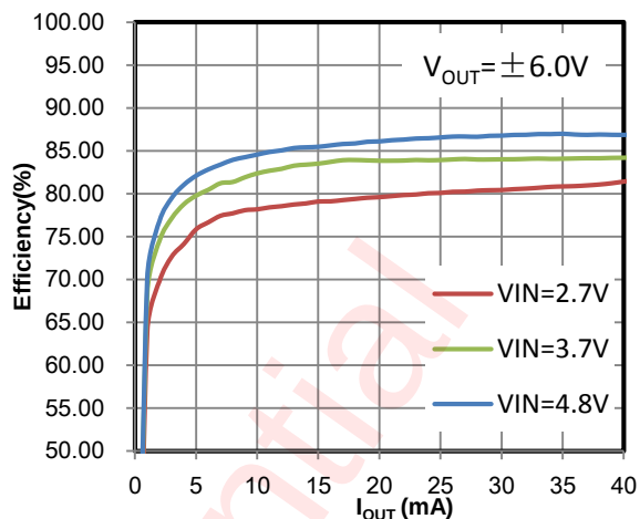
Figure 12 Efficiency (40mA Mode)
