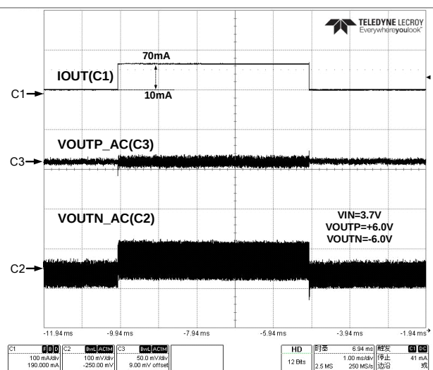
Figure 52 Load Transient (80mA Mode)
