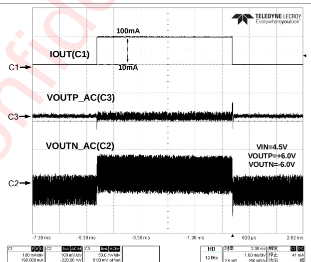
Figure 56 Load Transient (100mA Mode)
