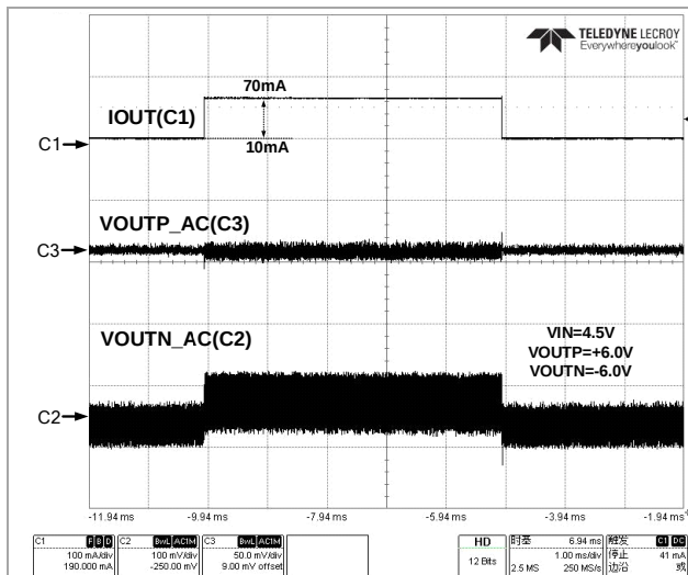
Figure 53 Load Transient (80mA Mode)
