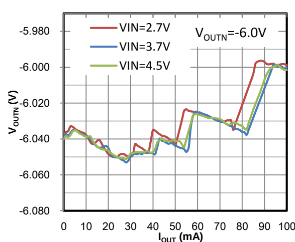
Figure 40 Load Regulation (100mA Mode)
