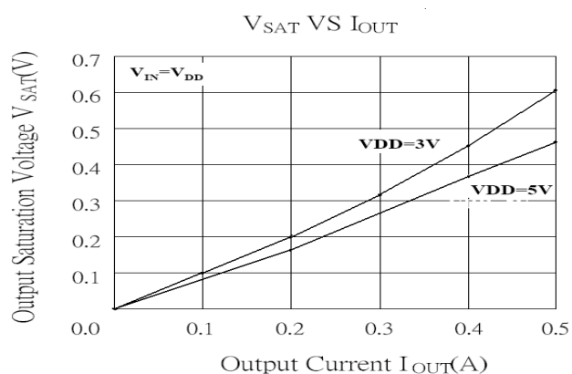
Figure 4a. V_{SAT} VS I_{OUT}
