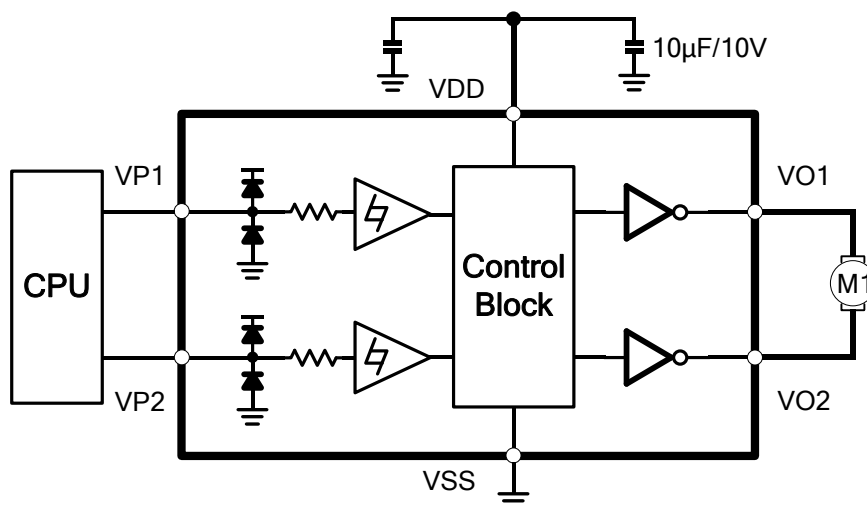
Figure 6. Typical DC Motor Application
