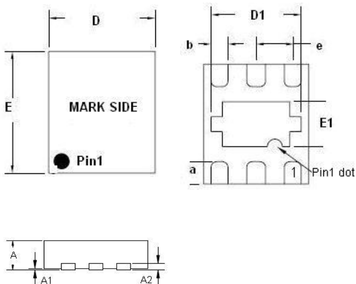
STDFN-6 1.4mm×1.6mm (Pitch: 0.5mm) Package (Unit: mm)
