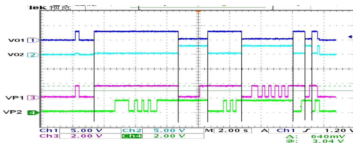
Figure 5. Truth Table test waves
