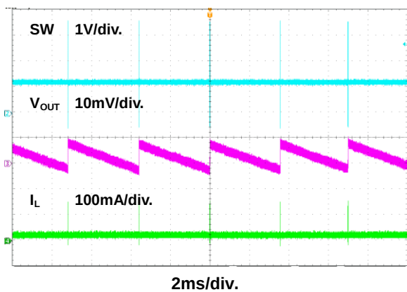
Figure 15. Switching Waveform
